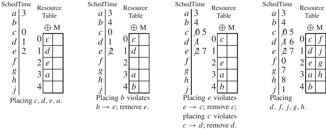
FIGURE 20.10. Iterative modulo scheduling applied to Program 20.4b. Graph 20.5a is the data-dependence graph; \Delta_{\min} = 5 (see page 451); H = [c, d, e, a, b, f, j, g, h] .
